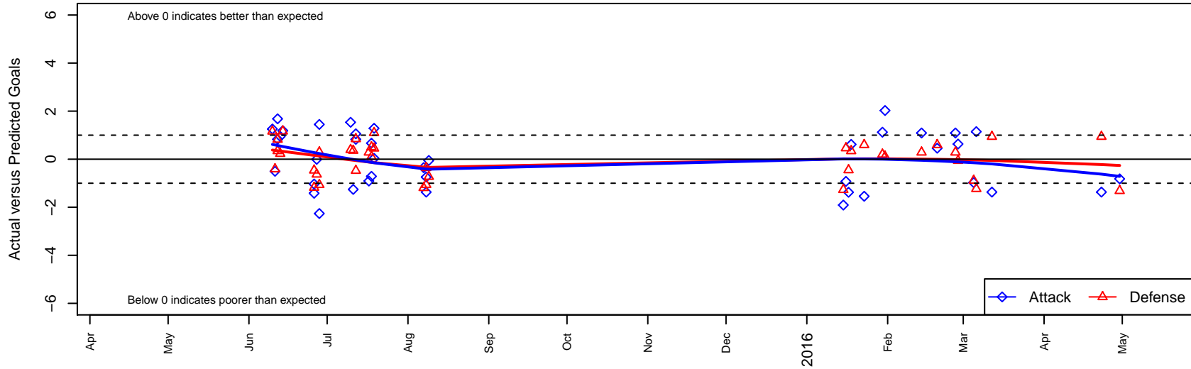
Washington Timbers Green G97 Dots are actual minus expected GF (blue circles) and GA (red triangles). Blue line is smoothed change in attack strength. Red is smoothed change in defense strength.
